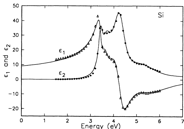
FIG. 7. The solid lines are the theoretical plots of \epsilon_1(E) = n^2(E) - k^2(E) and \epsilon_2(E) = 2n(E)k(E) , where n(E) and k(E) are given by Eqs. (19) and (15) with the parameters specified in Table II for crystalline Si. \epsilon_1 : \triangle and \epsilon_2 : \bullet experimental data are from Aspnes and Studna (Ref. 13).
