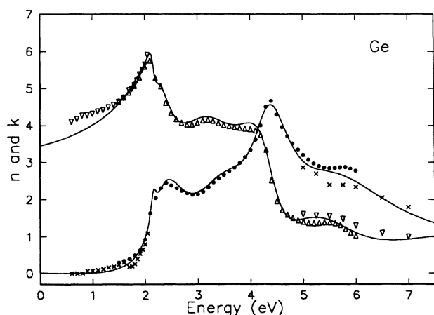
FIG. 8. The solid lines are the theoretical plots of n(E) and k(E) given by Eqs. (19) and (15) with the parameters specified in Table III for crystalline Ge. n : \triangle and k : \bullet experimental data are from Aspnes and Studna (Ref. 13). n : \nabla and k : \times experimental data are from Ref. 4.
