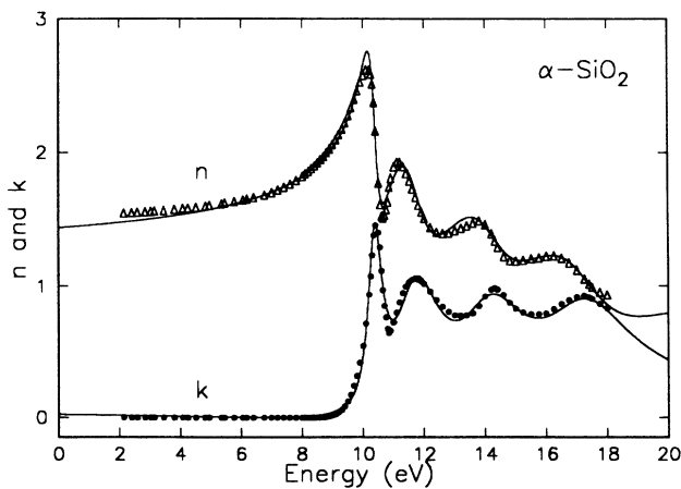
FIG. 5. The solid lines are the theoretical plots of n(E) and k(E) given by Eqs. (19) and (15) with the parameters specified in Table II for crystalline \alpha -SiO 2 . n : \triangle and k : \bullet experimental data are by Philipp (Ref. 16).
