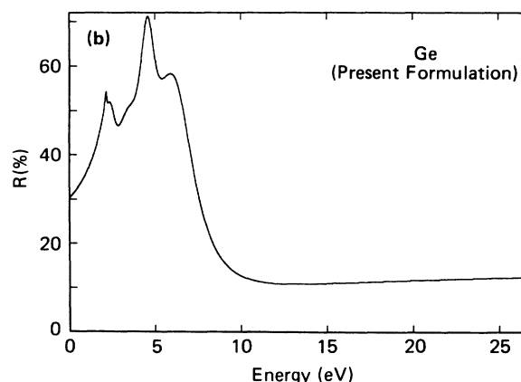
FIG. 9. (a) Experimental reflectance spectrum of crystalline Ge taken from Ref. 22. (b) Theoretical reflectance spectrum, R(E) = \{[n(E) - 1]^2 + k^2(E)\} / \{[n(E) + 1]^2 + k^2(E)\} , where n(E) and k(E) are given by Eqs. (19) and (15) with the parameters specified in Table III for crystalline Ge.
