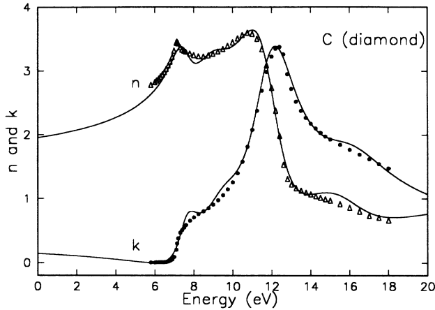
FIG. 4. The solid lines are the theoretical plots of n(E) and k(E) given by Eqs. (19) and (15) with the parameters specified in Table II for crystalline cubic C. n : \triangle and k : \bullet experimental data are by Philipp and Taft (Ref. 15).
